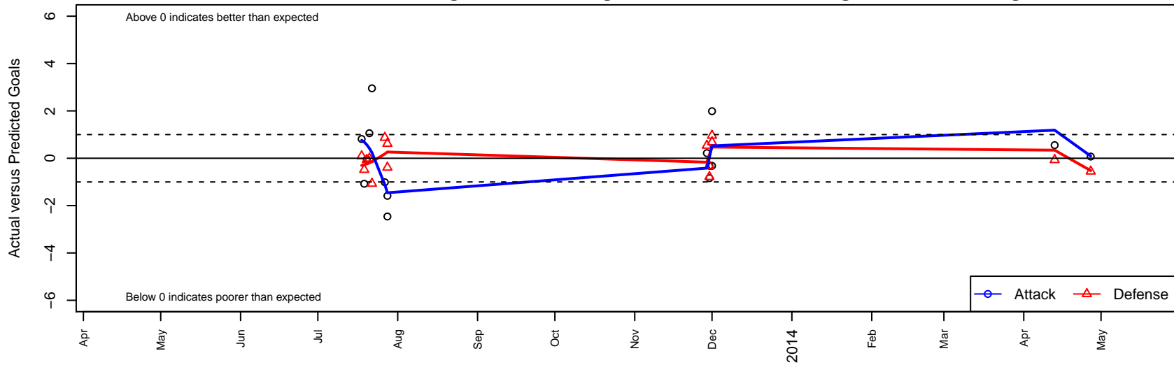
CZ Elite B95 Dots are actual minus expected GF (blue circles) and GA (red triangles). Blue line is smoothed change in attack strength. Red is smoothed change in defense strength.
